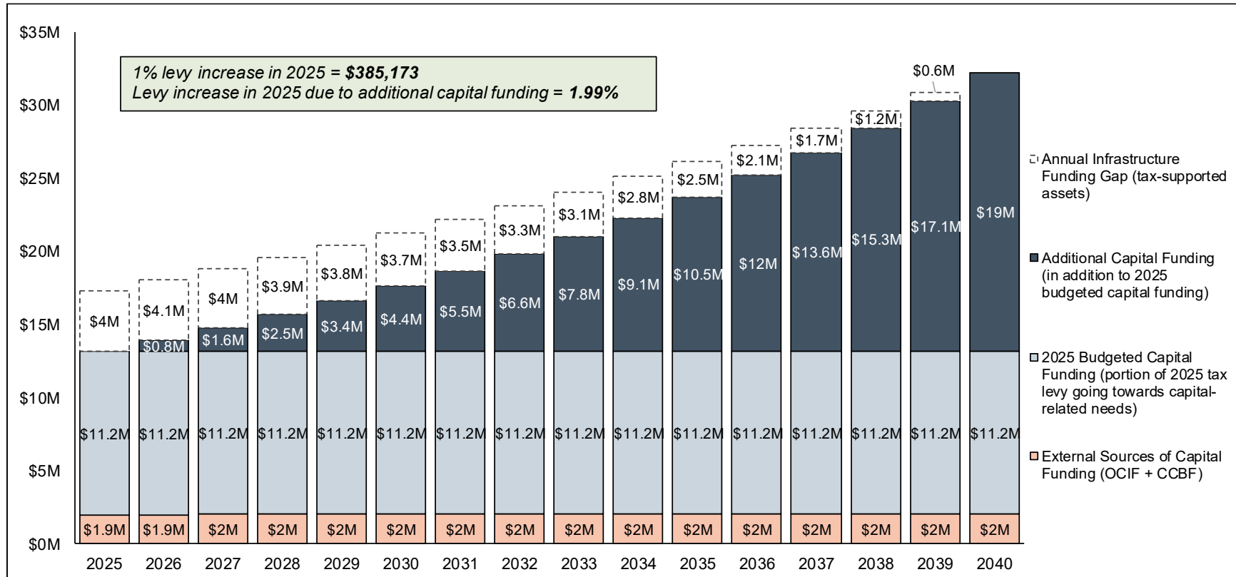
Figure 4-6: Tax-funded Assets – Capital Funding Forecast with 15-year Phase-in Period (Inflated)
